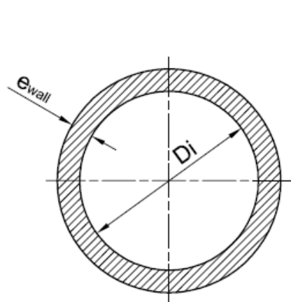
Figure 11 — Wall thickness calculation
