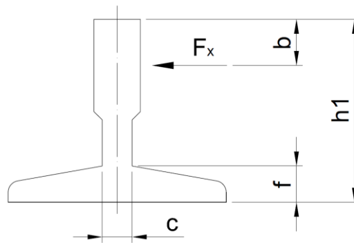
Figure 5 — Dimensions for flange bending calculation
