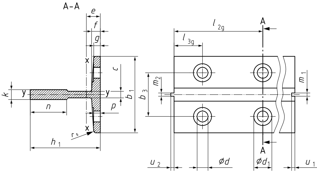
Figure 2 — Cold-drawn, inclined-foot flange guide rail
