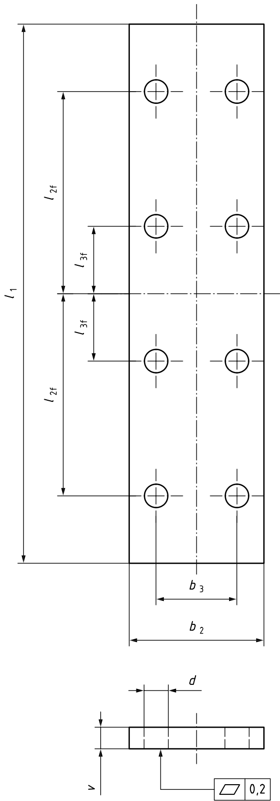
Figure 6 — Fishplate
