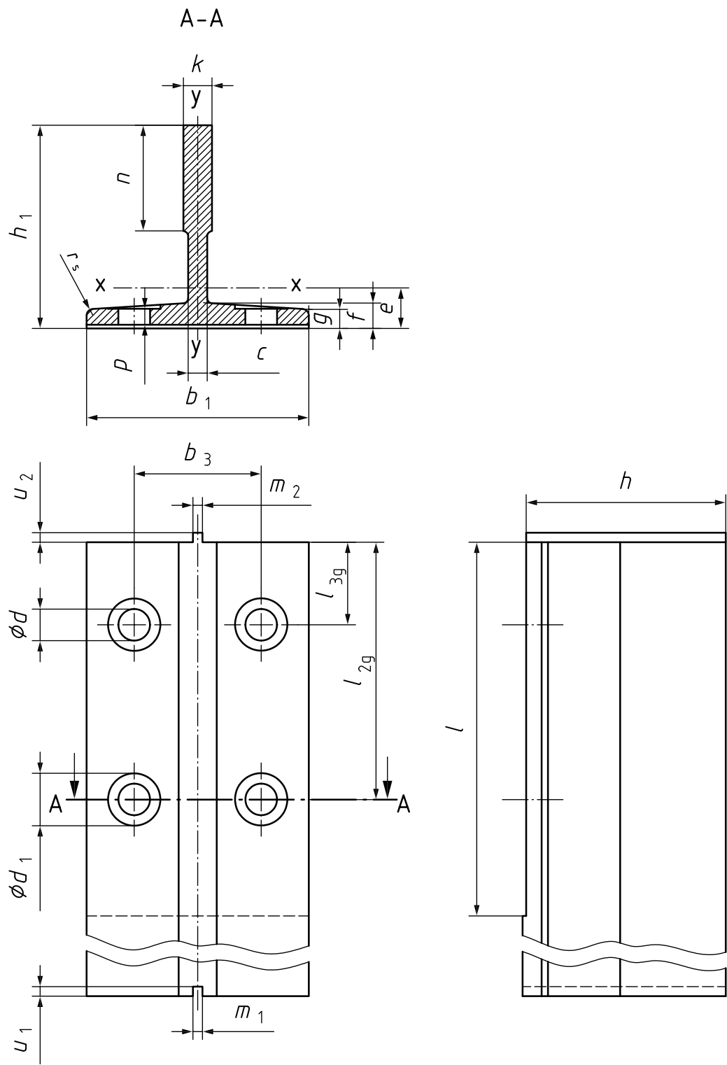
Figure 3 — Machined guide rail
