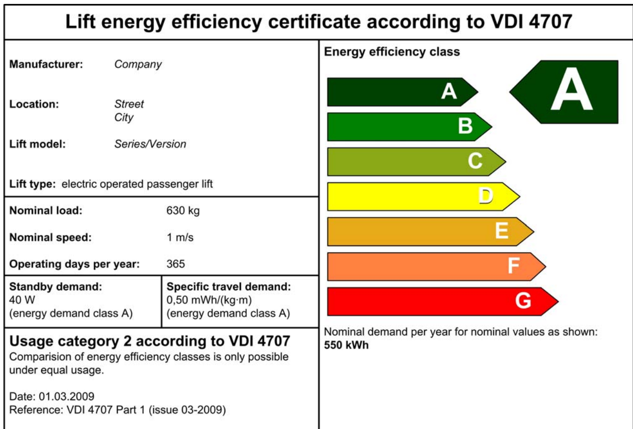
Figure 2. Energy certificate for a lift according to VDI 4707 Part 1
