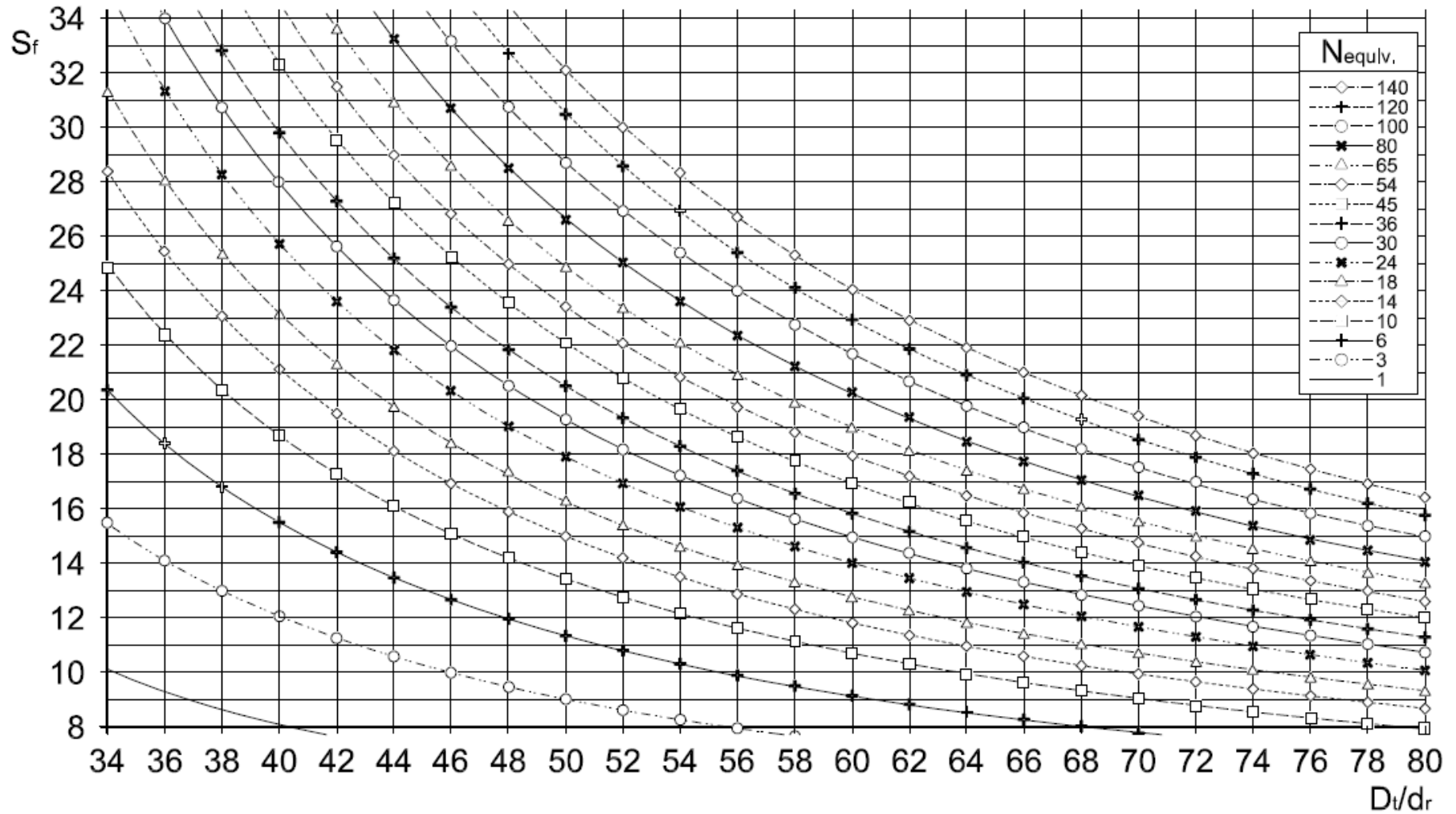
Figure 10 — Evaluation of minimum safety factor
