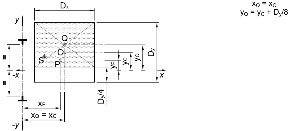
Figure C.3 — Safety gear operation - Load distribution in lift car – Case 2 relative to y-axis
