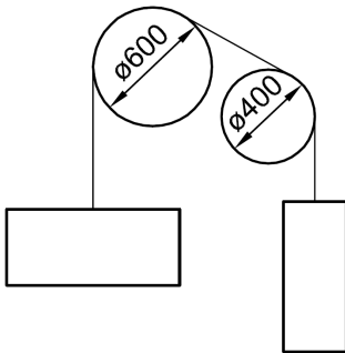
Figure E.1 — 2 to 1 roping - V grooves
