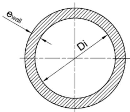
Figure 11 — Wall thickness calculation
