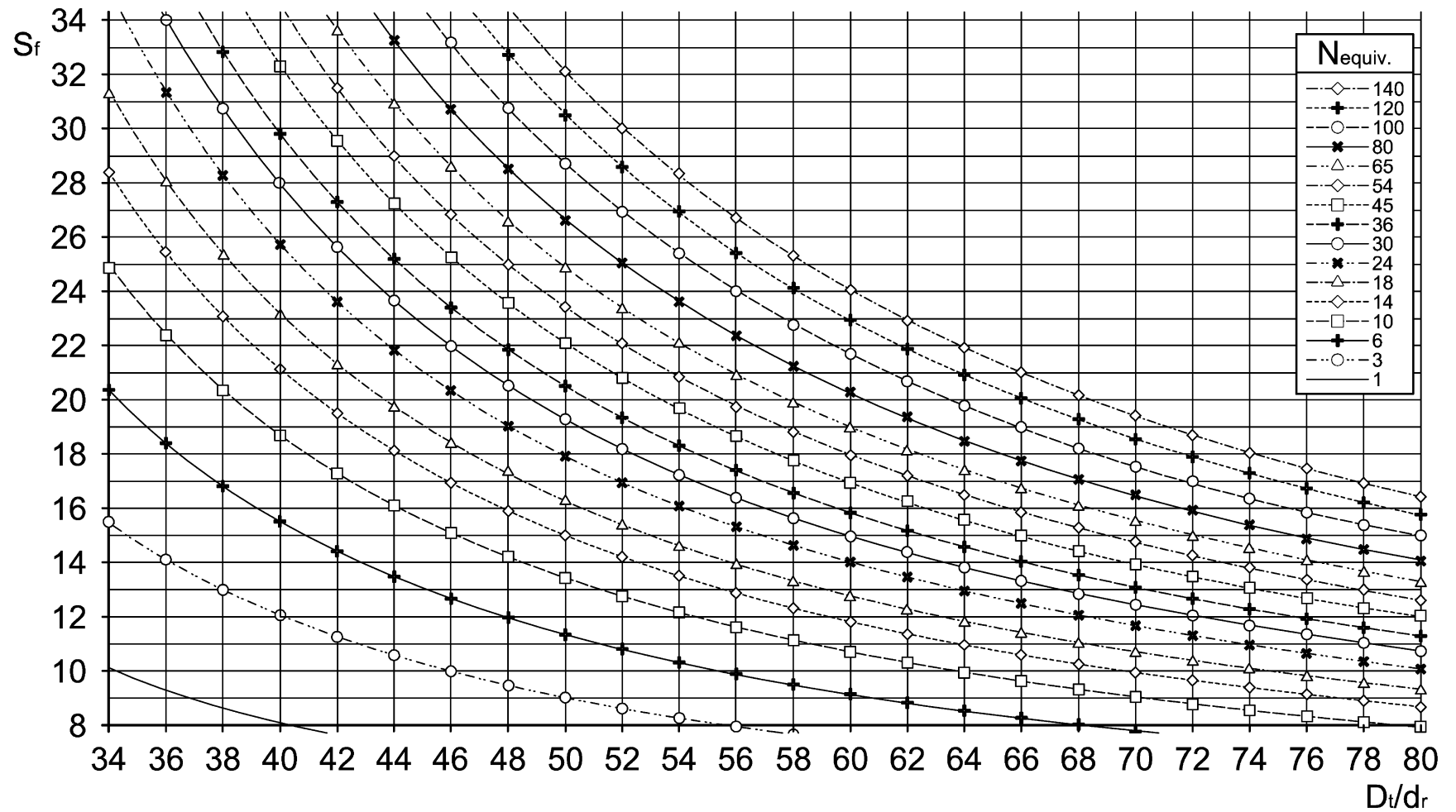
Figure 10 — Evaluation of minimum safety factor
