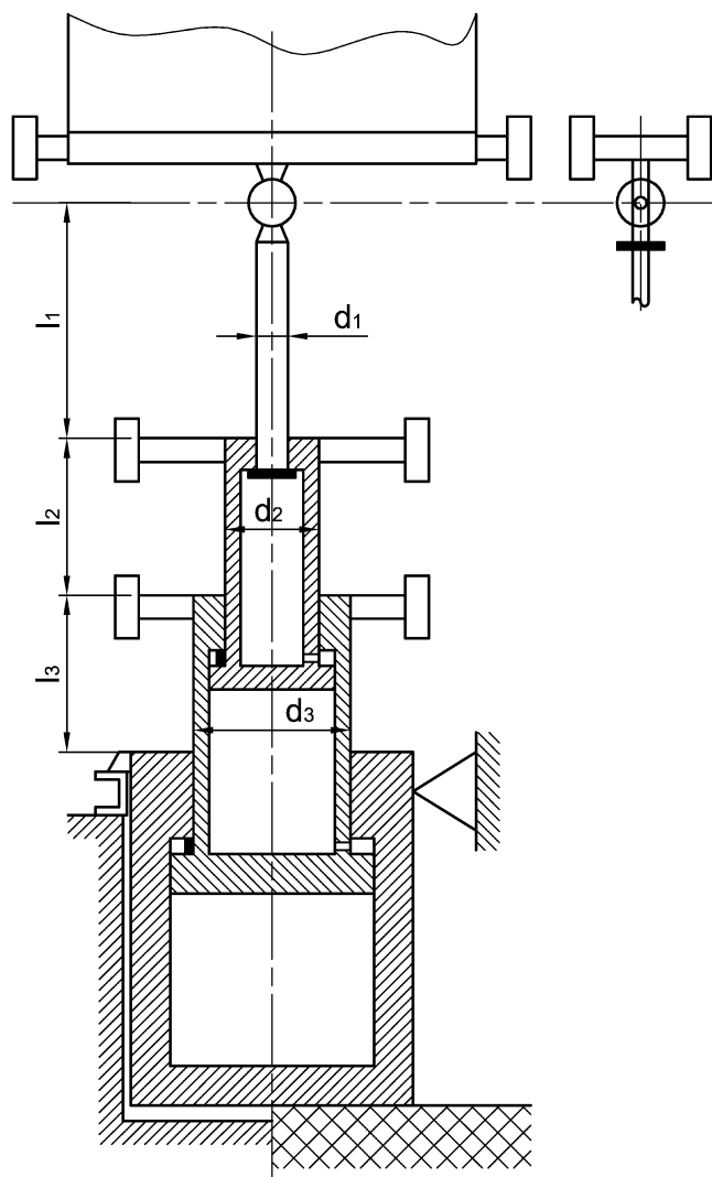
Figure 17 — Telescopic jacks with external guidance
