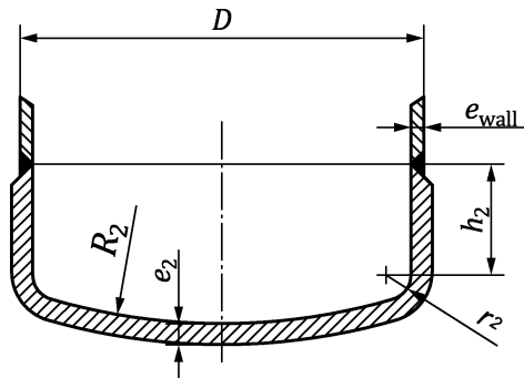
Figure 13 — Cambered based
